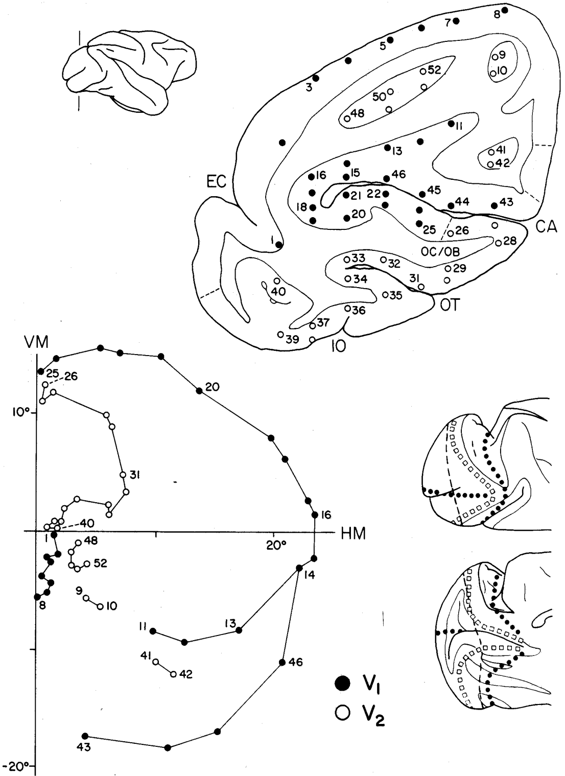
Fig. 8. Location of receptive field centers (lower left) in V1 and V2 recorded at the sites indicated in the coronal section (upper right). The drawings in the lower right show the vertical meridian (squares), the horizontal meridian
