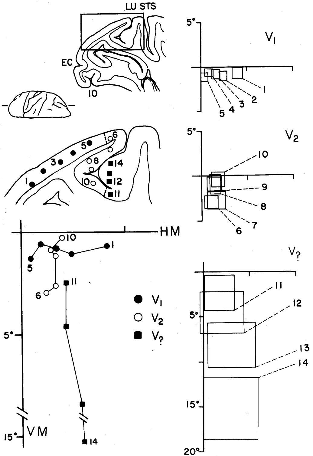
Fig. 5. Central receptive fields in dorsal V_1 , V_2 , and an area anterior to V_2 . The recording sites are indicated on the enlarged sagittal section (cut at the level indicated on the dorsal view of the brain). See also legend to Figures 1 and 4.
