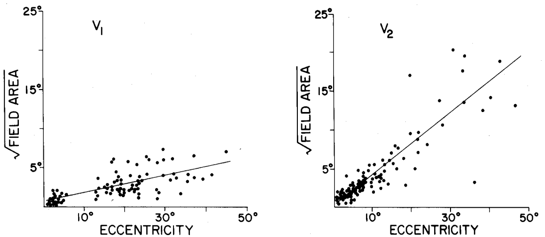
Fig. 13. Square root of receptive field area vs. retinal eccentricity for V1 (left) and V2 (right). Data for both areas were obtained from two animals. The straight lines were fitted with the method of least squares.
